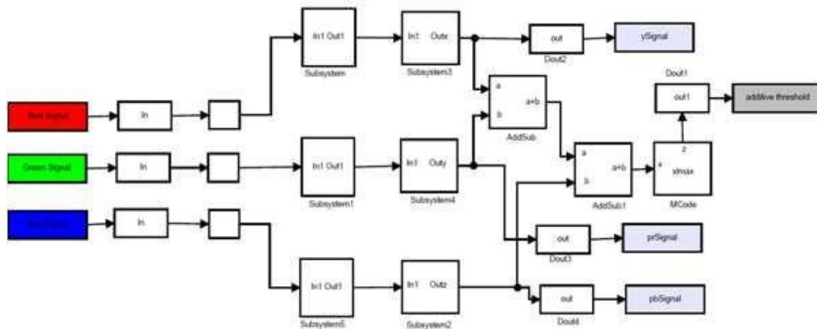
Fig 3: hardware architecture for image thresholding.
